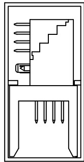
Drawing One: Product Installing Mode (圖一產品裝入方式)
