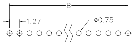
P.C. Board Layout
