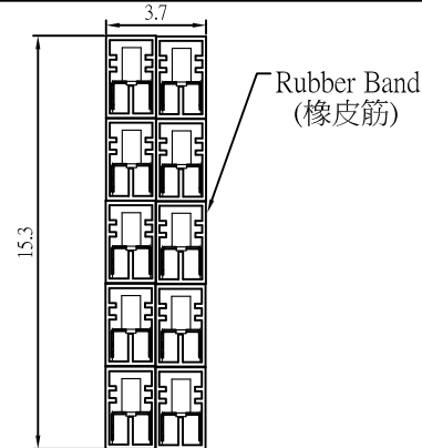
Drawing Two: Each Bundle 10 Tube (圖二: 每10管為1捆)
