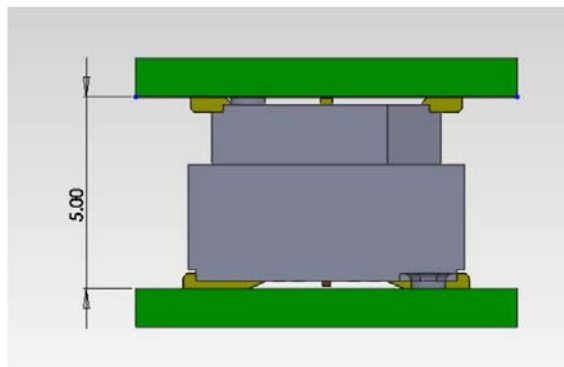
Distance between male's PCB and female's PCB is 5.00REF 公母PCB板之間的尺寸為5.00REF
