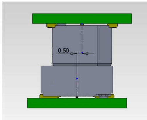
allowed misalignment in longitudinal axes 在縱向方向允許對插容差
