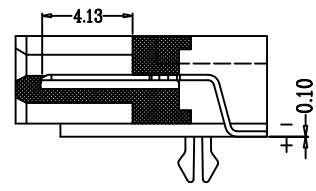
Sect B-B
