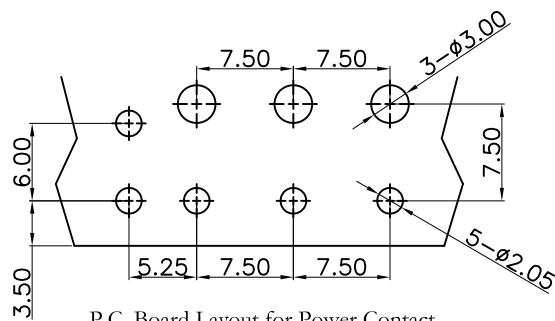
P.C. Board Layout for Power Contact
