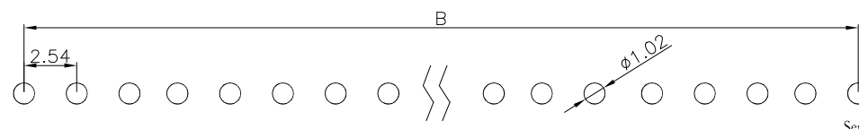
P.C. Board Layout
